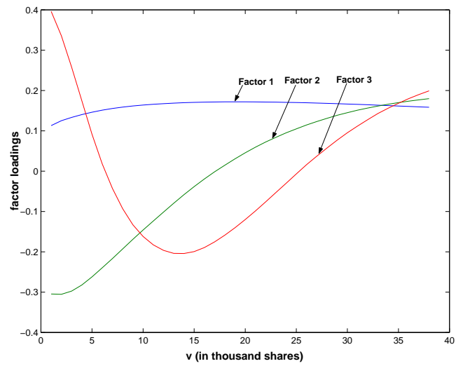
Figure 4: Factor loadings of first three principal components
