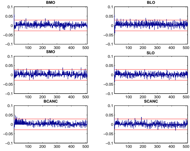
Figure 3: Autocorrelogram of the Pearson residuals - Aggregated MDACP system
