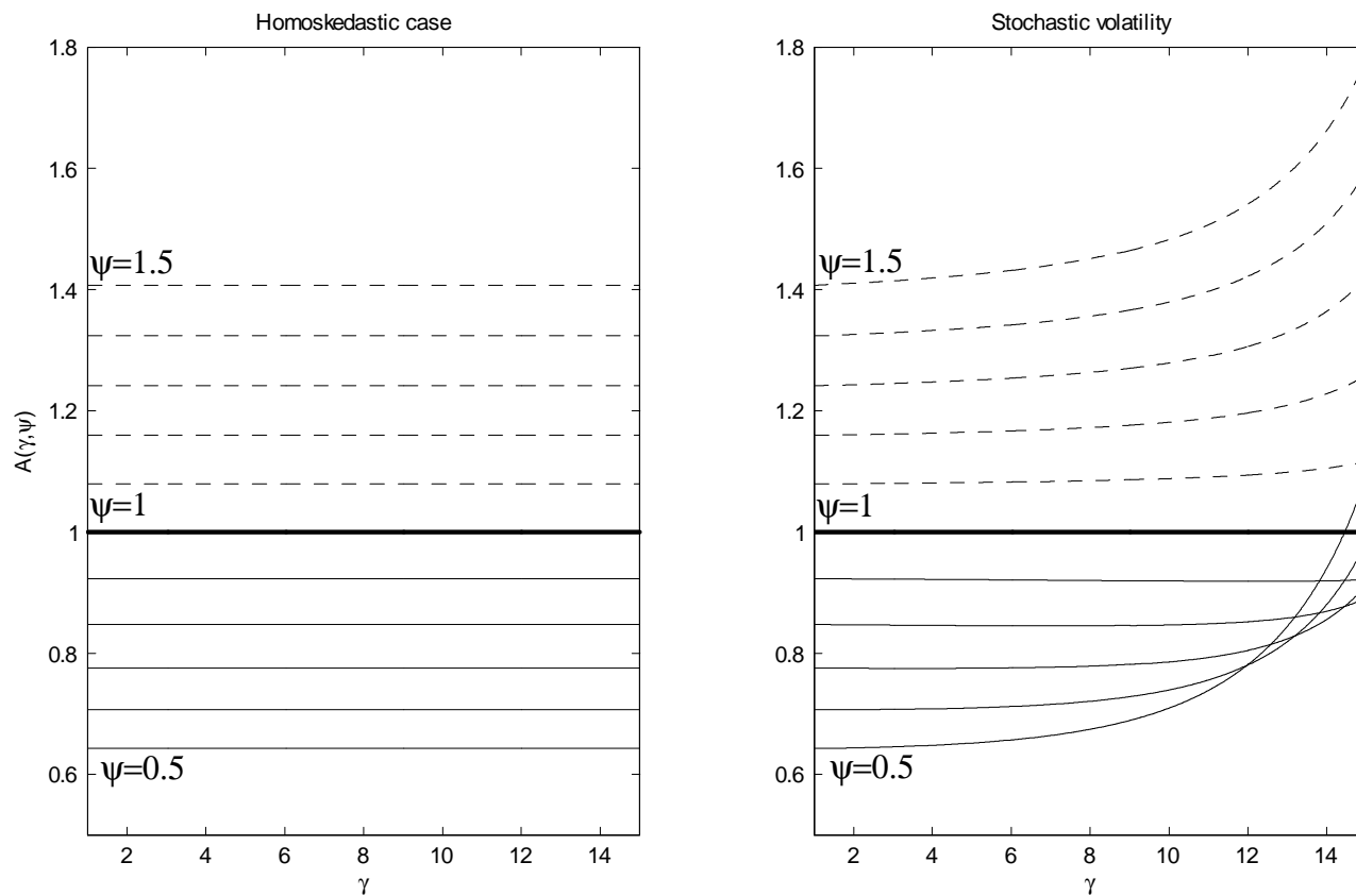
Figure 2: This figure plots plots the coefficient A(\gamma, \psi) relating the conditional volatility of consumption growth to the volatility of returns for different values of \gamma and \psi for the homoskedastic case (left panel) and for the heteroskedastic case (right panel), where A(\gamma, \psi) is a function of the variances and covariances of the scaled residuals u_{t+1} . In each panel, we plot A(\gamma, \psi) as \gamma varies between 1 and 15, for different values of \psi . Each line corresponds to a different \psi between 0.5 and 1.5.
